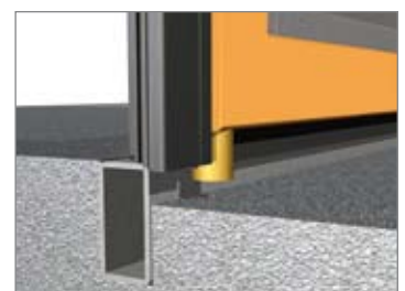
bottom rail with stop
