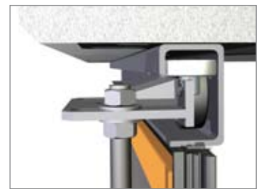
running rail profile – in embasure
