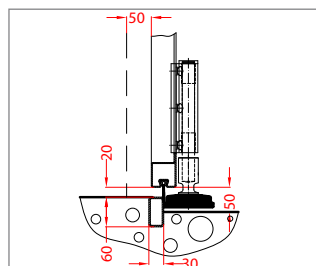
Bodenschiene bottom rail with stop
