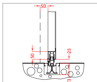
Bodenschiene recessed bottom rail with carrier roller
