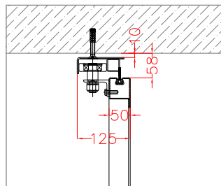
Laufschiene in Laibung running rail – in embrasure
