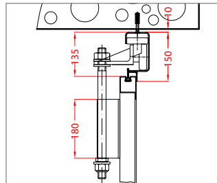
Laufschiene in Laibung running rail profile – in embrasure
